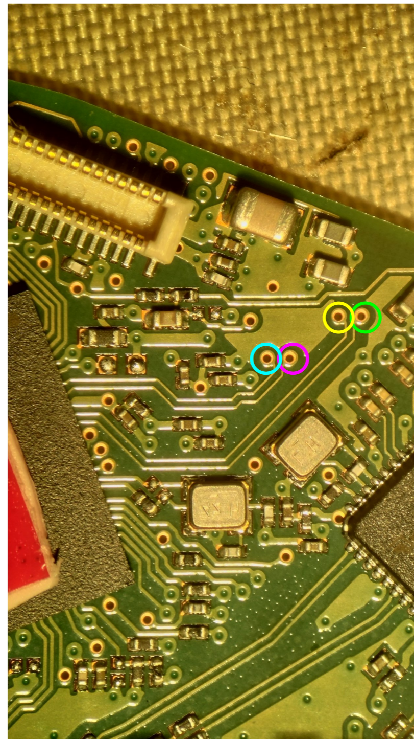
Mirror (soldering side)
